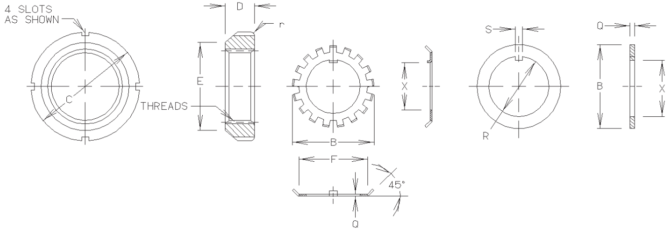
Figure 1 – Locknuts
